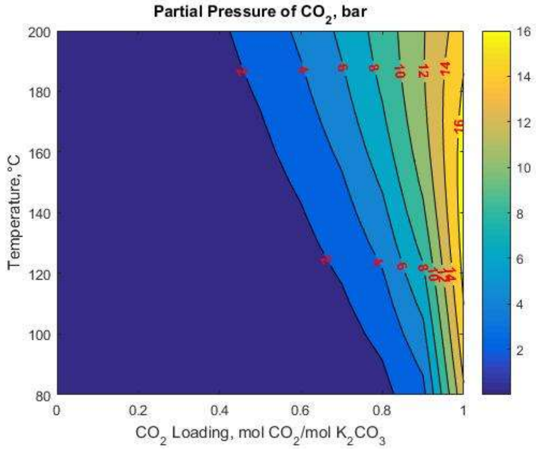
Figure 4.2. Partial pressure of CO 2 at a temperature of 80 – 200°C and CO 2 loading from 0 – 1.0.
